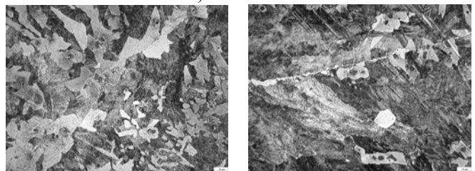
b) Modified with \text{FeSi}_{34}\text{V}_{25}\text{Ti}_{12}
