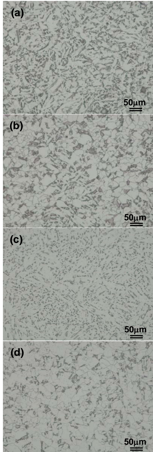
Fig. 6 Optical microstructures observed after hot compression tests. Steel A compressed under the strain rate of 1 s^{-1} at temperatures of (a) 900°C and (b) 1050°C. Steel B compressed under strain rates of (c) 1 s^{-1} and (d) 5 s^{-1} , and at the temperature of 1000°C
