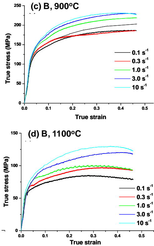
Fig. 2 True stress-true strain curves obtained at temperatures of 900°C (a, c) and 1100°C (b, d) under the various strain rates
