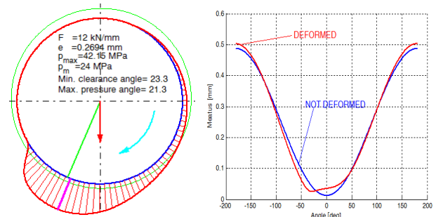
Fig. 5 Pressure distribution for JB1 configuration ( \alpha=0 , T_{in}=40^\circ\text{C} – T_{out}=80^\circ\text{C} ) with deformable components (left). Lubrication gap for rigid and deformable components (right)
