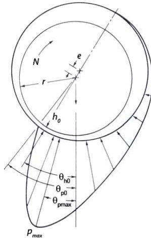
Fig. 1 Sketch of a hydrodynamic journal bearing
