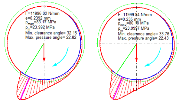
Fig. 2 Results for JB1 configuration (linear temperature variation, T_{in}=40^{\circ}\text{C} - T_{out}=80^{\circ}\text{C} ), with \alpha=0 (left) and \alpha=0.01 (right)
