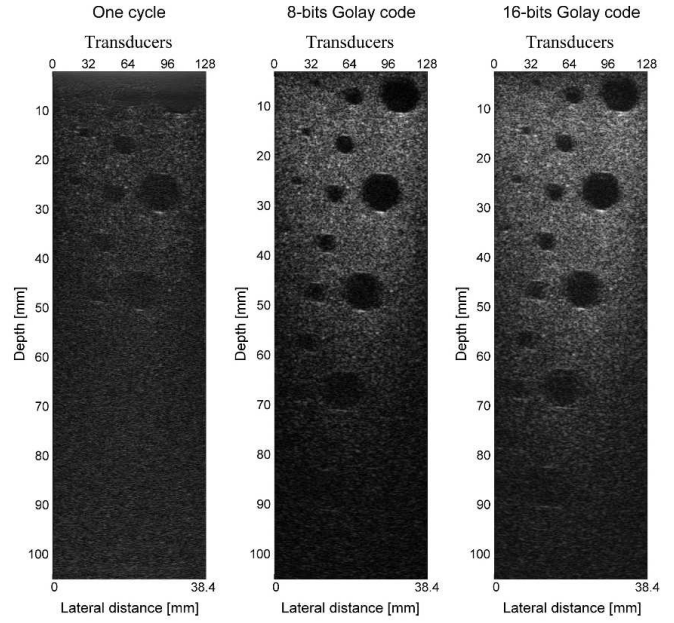
Fig. 10 2D ultrasound images of cyst phantom using: a) one cycle; b) 8-bit Golay code; c) 16-bit Golay code
