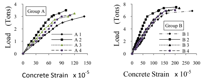
Fig. 7 Load-Concrete strain diagram for tested beams
