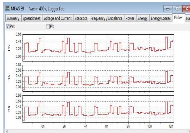
Fig. 3 Flicker level in Al-Nasim Dairy
