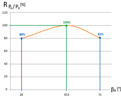
Fig. 8 Power relations of collectors in autumn, \beta_B = 47.5^\circ
