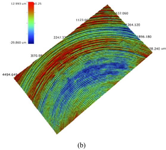
Fig. 4 (a) SEM and (b) optical profiler images of plasma treated VEUHMWPE-1 worn surfaces
