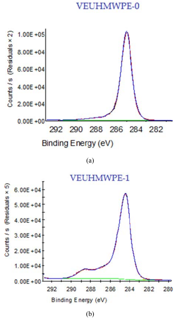
Fig. 6 X-ray photoelectron spectroscopy spectrum of VEUHMWPE: (a) High resolution XPS C1s peaks of VEUHMWPE-0 (untreated sample) and (b) VEUHMWPE-1 (plasma treated sample)
