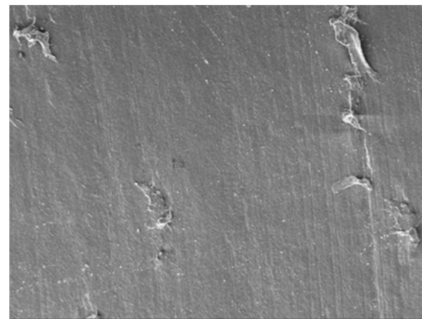
Fig. 3 (a) SEM and (b) optical profiler images of untreated VEUHMWPE-0 worn surfaces
