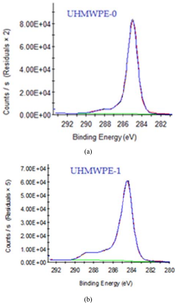
Fig. 5 X-ray photoelectron spectroscopy spectrum of UHMWPE: (a) High resolution XPS C1s peaks of UHMWPE-0 (untreated sample) and (b) UHMWPE-1 (plasma treated sample)
