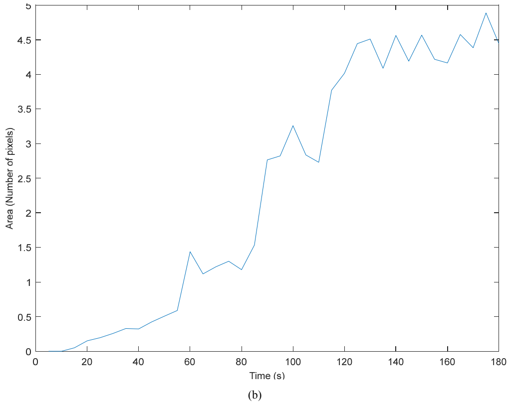
Fig. 10 Spark evolution (a) intensity, and (b) area
