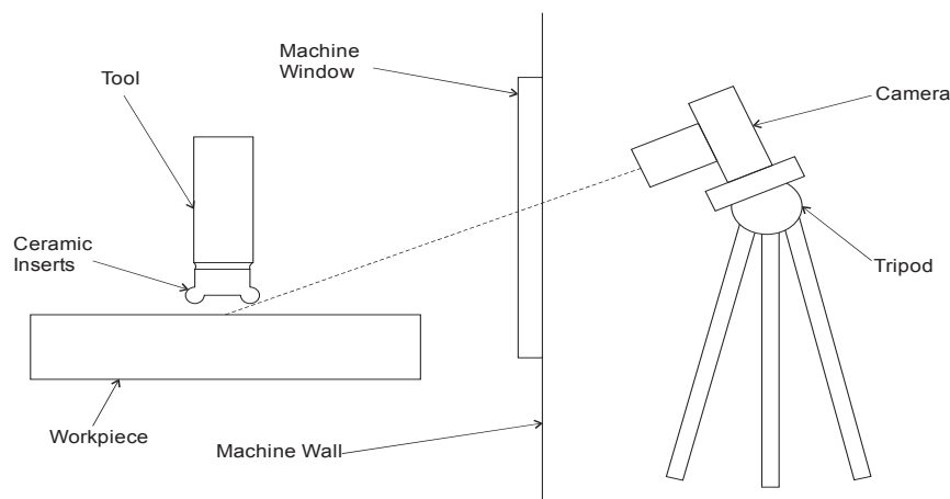
Fig. 2 Camera set-up
