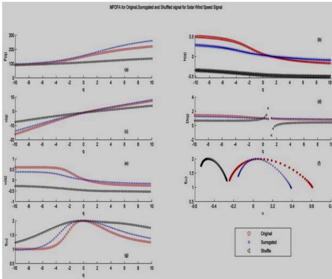
Fig. 5 Comparative view of the plots for original, surrogated and shuffled time series data: (a) F(q) against q , (b) h(q) against q , (c) \tau(q) against q , (d) D(q) against q , (e) \alpha(q) against q , (f) f(\alpha) against \alpha , (g) f(\alpha) against q
