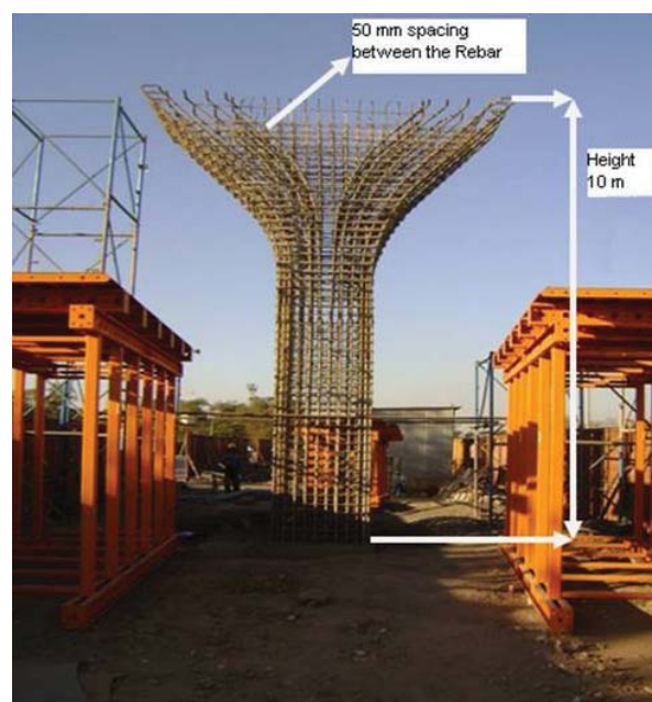
Fig. 2 Typical column detailing of Mumbai Monorail piers
