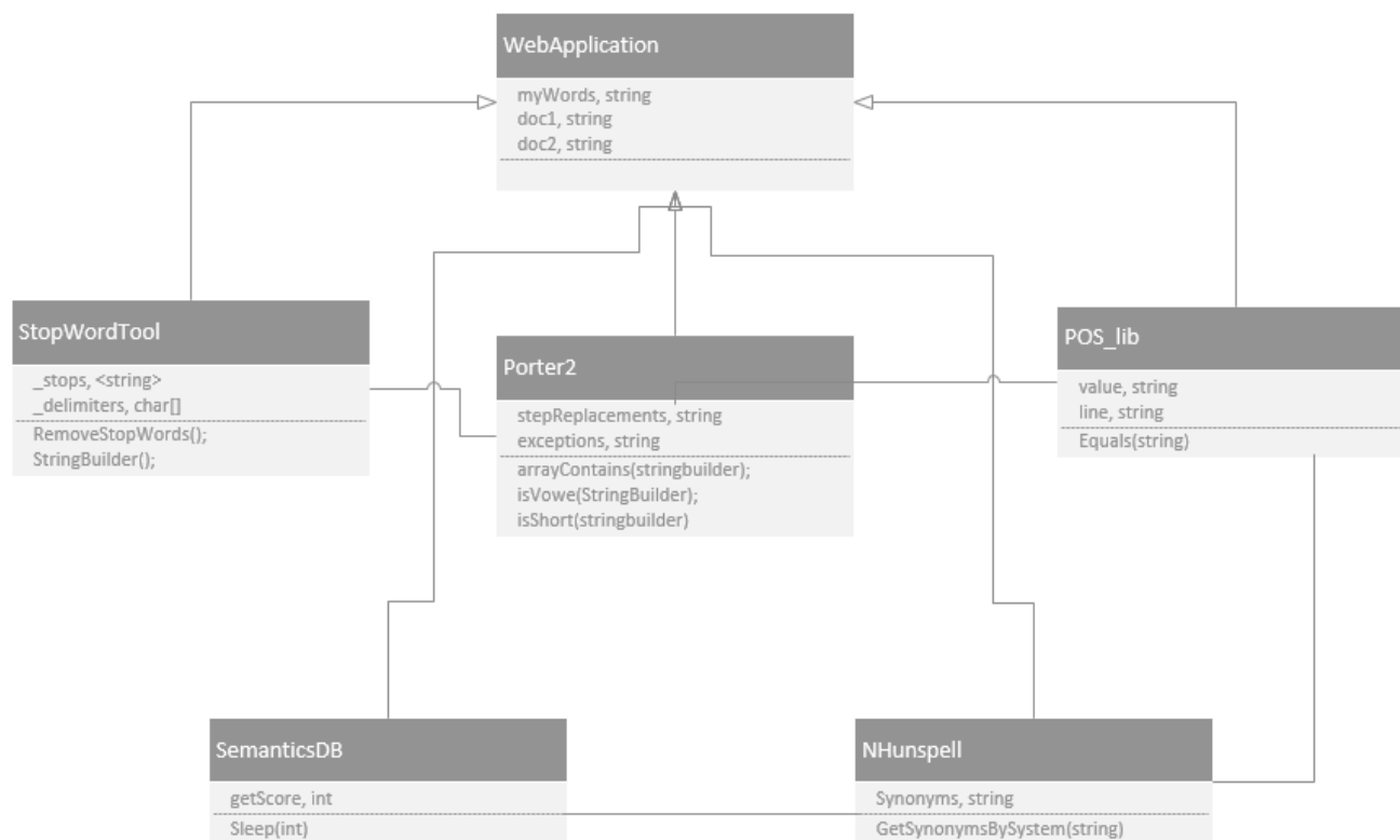
Fig. 1 Class Diagram
