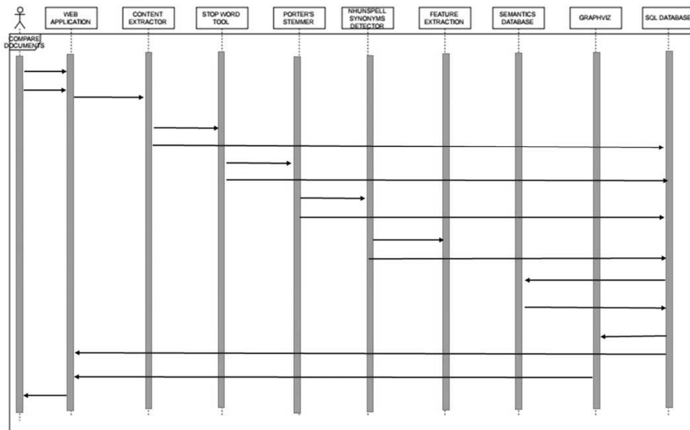
Fig. 2 Workflow diagram
