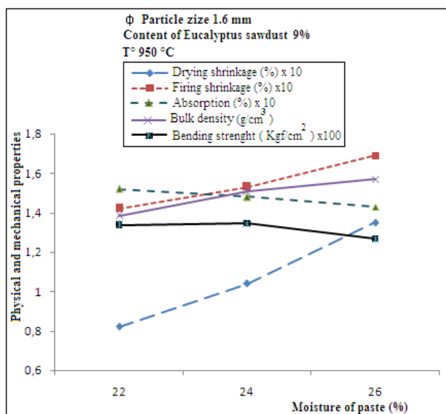
Fig. 2 Physical-mechanical properties in relation with moisture of mixtures according the particle size and Eucalyptus content
