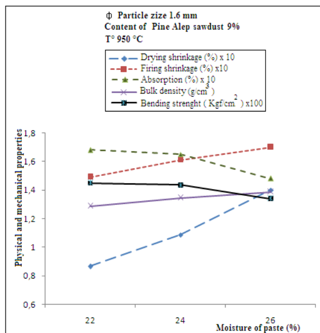
Fig. 3 Physical-mechanical properties in relation with moisture of mixtures according the particle size and Pine Alep content
